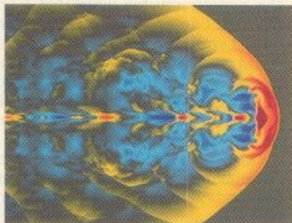
A supersonic gas jet. The colors display a logarithm of the pressure.
