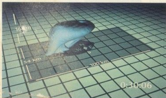
Simulation of a thunderstorm cloud after 30 minutes of development.
