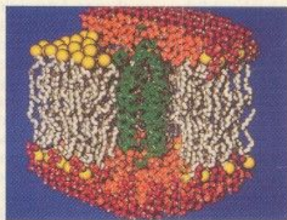
The bacteriorhodopsin protein (green) spans the cell membrane, as computed in a molecular dynamics simulation.
