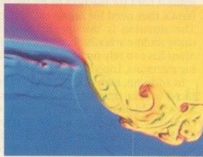
Strong waves roll up as the magnetized solar wind digs down into the Venusian ionosphere.
