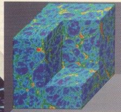
A volumetric visualization of the density of luminous matter in the universe.
