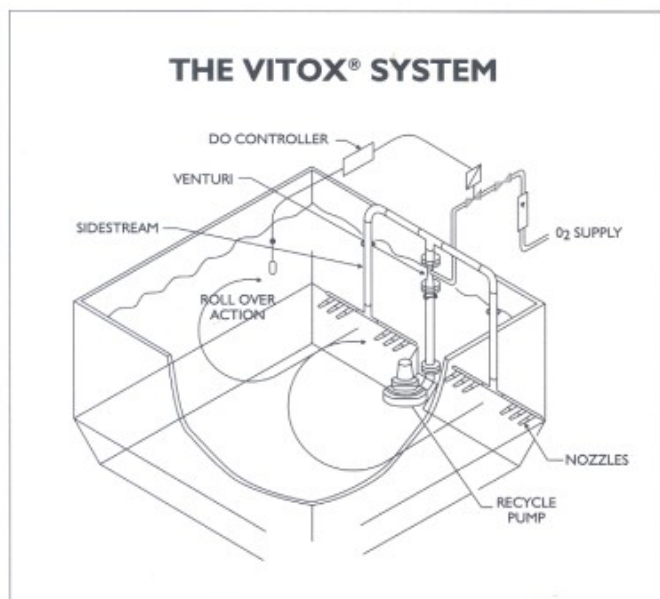
Simple to install and operate, the Vitox® sidestream system automatically controls dissolved oxygen in activated sludge basins.
